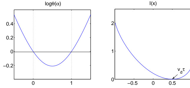
Figure 1: The cumulant generating function and the large deviation rate function.
